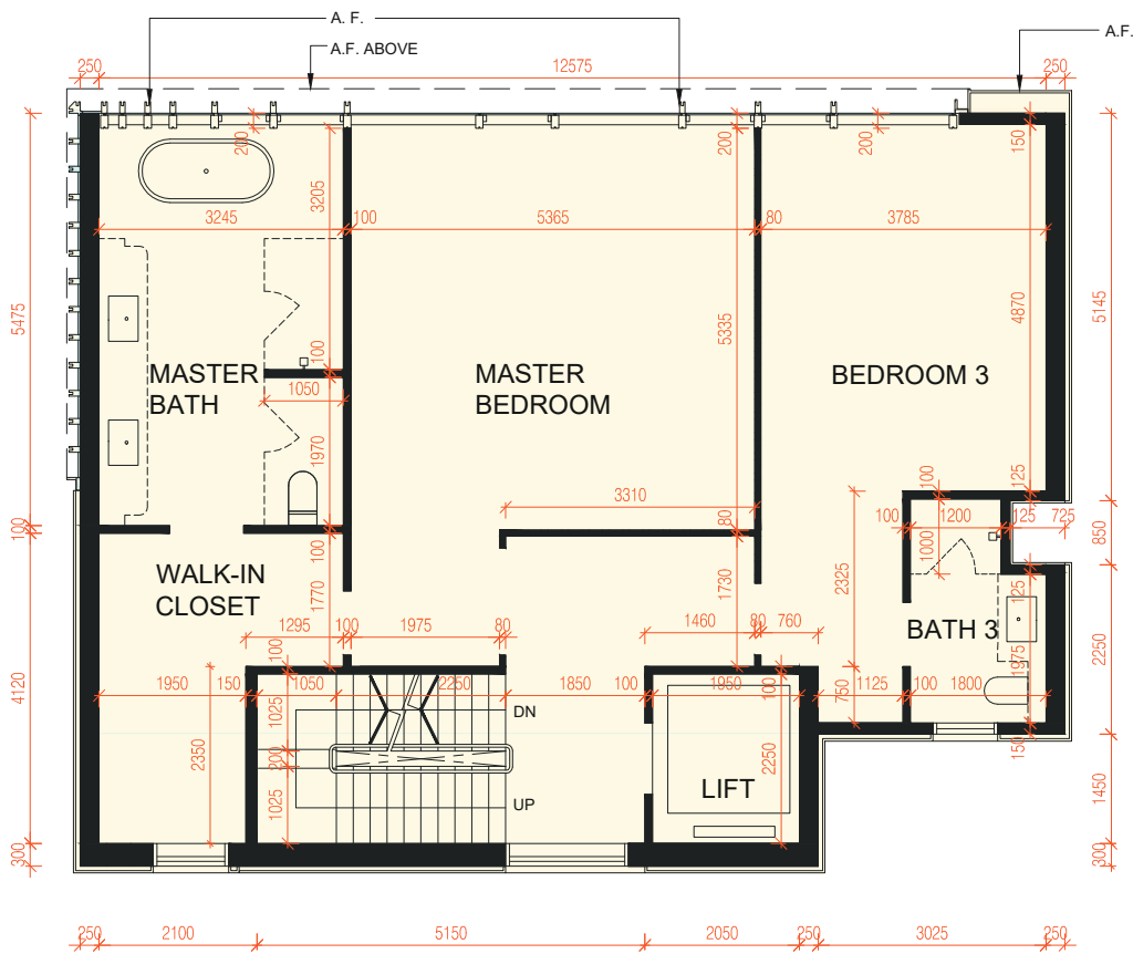
SECOND FLOOR PLAN 2樓平面圖
